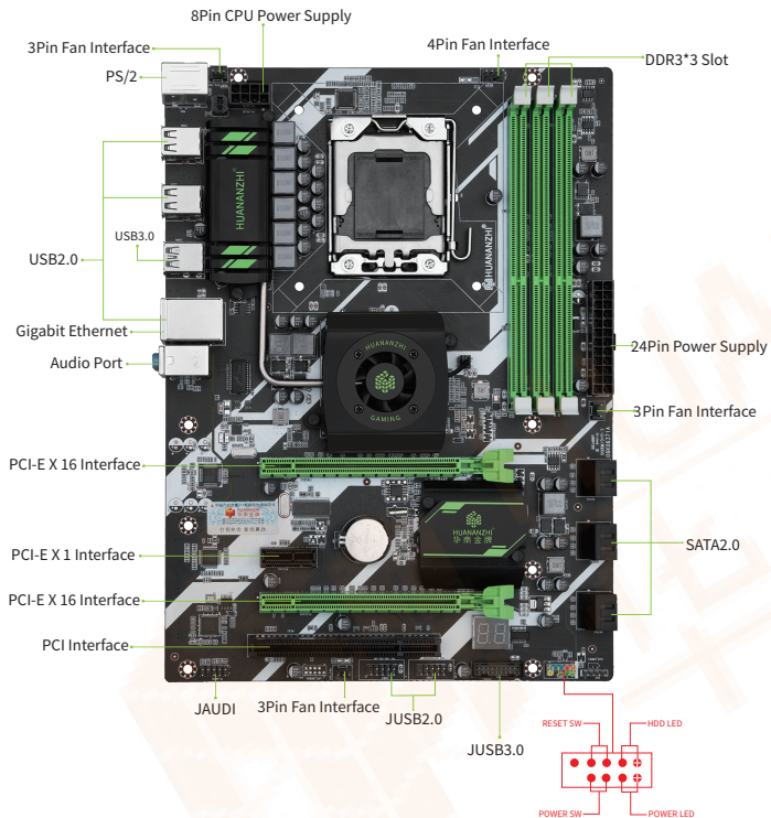
1-1 X58 DELUXE motherboard illustration
